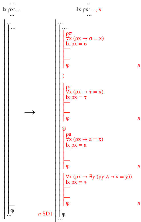
Fig. 8.6.3-1. Developing a derivation at stage n by securing a definite description; the independent term a is new to the derivation and the terms \sigma, \dots, \tau include at least one from each current alias set for the gap.
