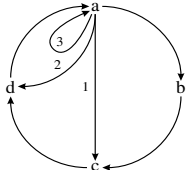
Fig. 7.8.2-2. A circuit from a to a reduced to a looped arrow in three steps by spanning linked arrows.
