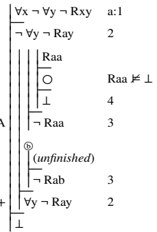
Fig. 7.8.1-1. Developing a derivation at stage n by planning for an unrestricted universal; the independent term a is new to the derivation and the terms \sigma, \tau, \dots, u include at least one from each current alias set for the gap.
