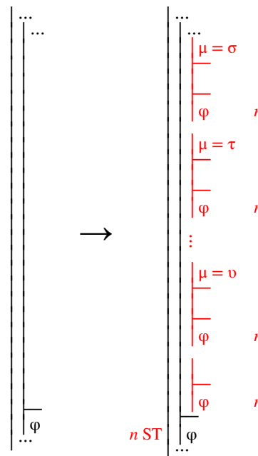
Fig. 7.8.1-2. Developing a derivation at stage n by securing a compound term \mu ; the terms \sigma, \tau, \dots, v include at least one from each current alias set for the gap other than the one including \mu .
