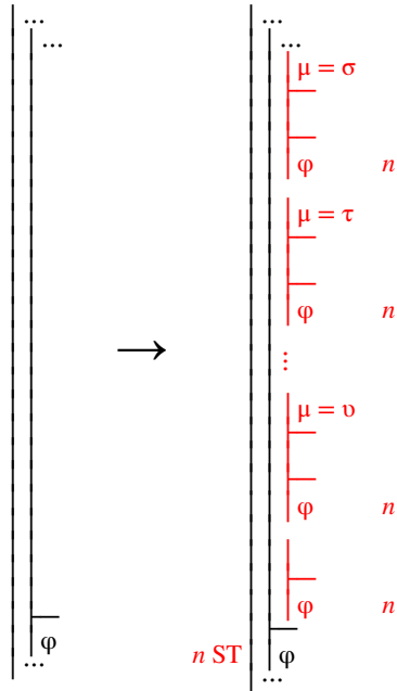
Fig. 7.8.1-2. Developing a derivation at stage n by securing a compound term \mu ; the terms \sigma , \tau , ..., \nu include at least one from each current alias set for the gap other than the one including \mu .
