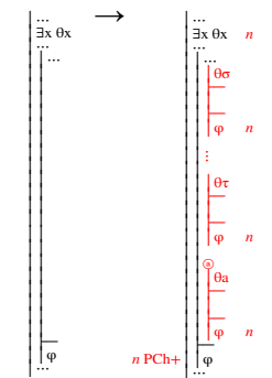
Fig. 8.5.3-4. Developing a derivation at stage n by exploiting an unrestricted or a restricted existential; the independent term a is new to the derivation and the terms \sigma, \dots, \tau include at least one from each current alias set for the gap
