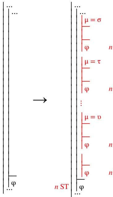
Fig. 7.8.1-2. Developing a derivation at stage n by securing a compound term \mu ; the terms \sigma , \tau , ..., \upsilon include at least one from each current alias set for the gap other than the one including \mu .
