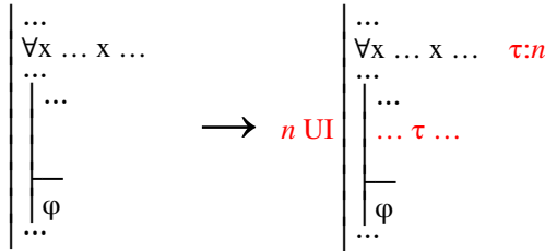
Fig. 7.5.4-2. Developing a derivation at stage n by exploiting an unrestricted universal for a term \tau .
