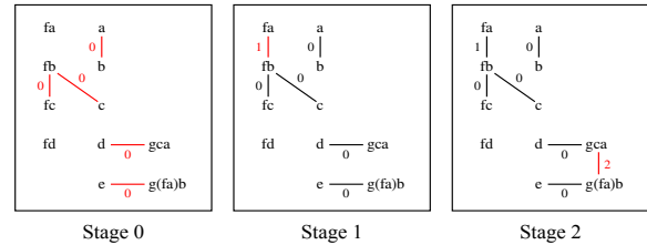
Fig. 6.3.2-3. Terms classified as co-aliases in a series of stages.
