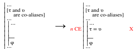
Fig. 6.3.3-5. At stage n , adding an equation between terms that are co-aliases with respect to the available resources.
