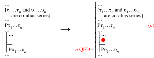
Fig. 6.3.3-3. Closing a gap one of whose resources differs from its goal only by terms that are co-aliases.
