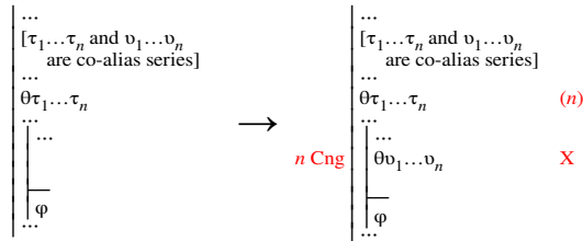
Fig. 6.3.3-6. At stage n , that differs from an available resource only by the occurrence of terms that are co-aliases.
