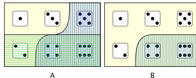
Fig. 5.2.3-1. Propositions expressed by two sentences (A) and an unless -conditional (B) whose main clause rules out the possibilities at the right in A.
