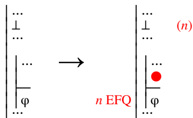
Fig. 2.2.6-2. Closing a gap that has \perp among its resources.
