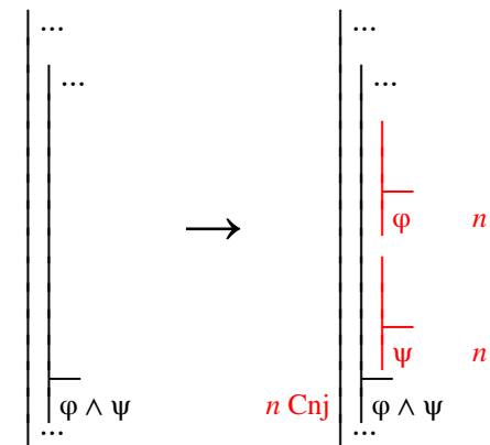
Fig. 2.2.3-2. Developing a derivation by planning for a conjunction at stage n . On the left, no assumptions are made about the resources, but the goal is
