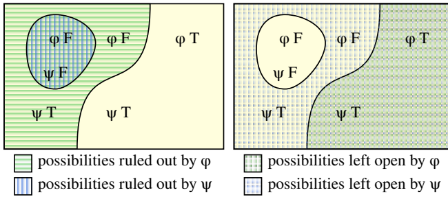
Fig. 1.2.3-1. The relation between non-equivalent propositions \phi and \psi where \phi \models \psi , depicted (on the left) by indicating the relation between the possibilities ruled out and (on the right) by indicating the possibilities left open by \phi and \psi .
