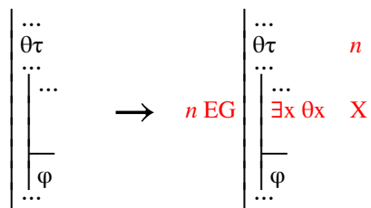
Fig. 8.5.3-3. Developing a derivation at stage n by adding an unrestricted existential that has an instance among the active resources.
