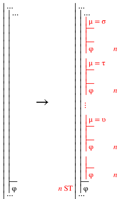
Fig. 7.8.1-2. Developing a derivation at stage n by securing a compound term \mu ; the terms \sigma, \tau, \dots, \upsilon include at least one from each current alias set for the gap other than the one including \mu .
