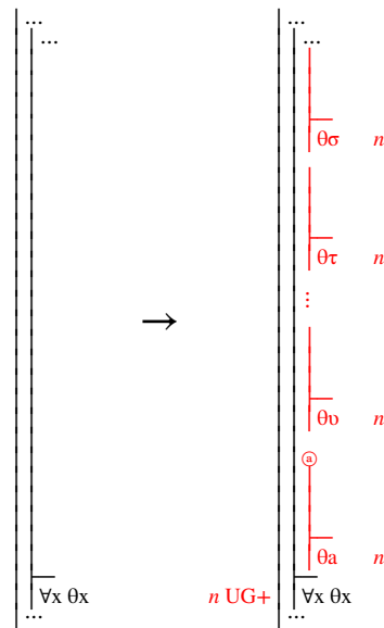
Fig. 7.8.1-1. Developing a derivation at stage n by planning for an unrestricted universal; the independent term a is new to the derivation and the terms \sigma, \tau, \dots, v include at least one from each current alias set for the gap.
