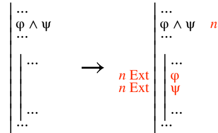
Fig. 2.2.3-1. Developing a derivation by exploiting a conjunction at stage n .
