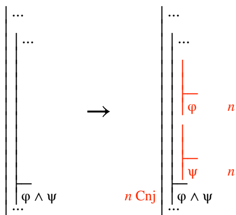
Fig. 2.2.3-2. Developing a derivation by planning for a conjunction at stage n . On the left, no assumptions are made about the resources, but the goal is shown
