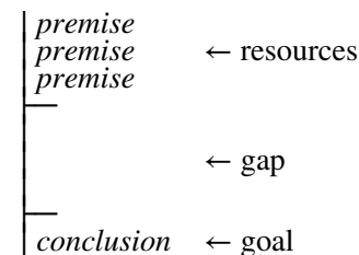
Fig. 2.2.2-1. The initial state of a derivation.
