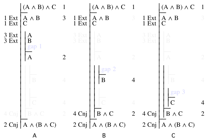
Fig. 2.2.7-2. A derivation from the perspective of each of its three gaps.
