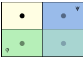
Fig. 1.2.5-1. The possibilities (the shaded bottom and right halves) that are ruled out by two propositions.
