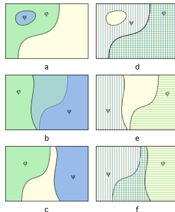
Fig. 1.2.6-1. Three relations between sentences \varphi and \psi . (a, d) \varphi implies \psi . (b, e) \varphi and \psi are mutually exclusive. (c, f) \varphi and \psi are jointly exhaustive. Regions ruled out by sentences are shaded in the top row—in green for \varphi and in blue for \psi . The regions left open are hatched in the bottom row—hatched horizontally for \varphi and vertically for \psi .
