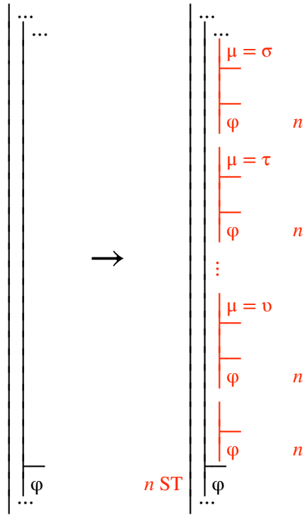
Fig. 7.8.1-2. Developing a derivation at stage n by securing a compound term \mu ; the terms \sigma, \tau, \dots, \nu include at least one from each current alias set for the gap.
