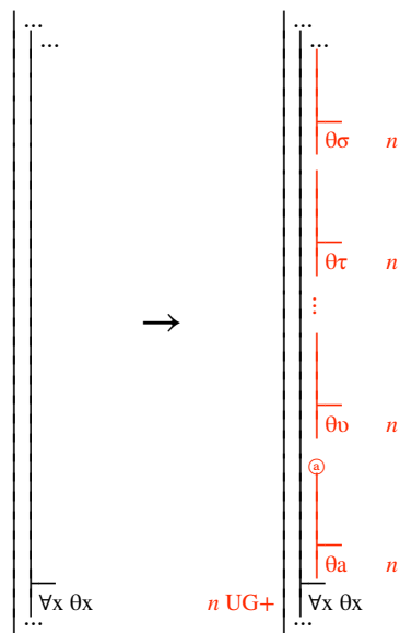
Fig. 7.8.1-1. Developing a derivation at stage n by planning for an unrestricted universal; the independent term a is new to the derivation and the terms \sigma, \tau, \dots, v include at least one from each current alias set for the gap.
