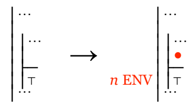
Fig. 2.2.5-1. Closing a gap that has ⊤ as its goal.
