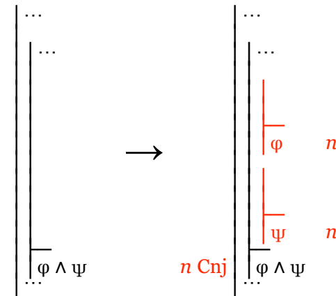
Fig. 2.2.3-2. Developing a derivation by planning for a conjunction at stage n .
