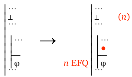
Fig. 2.2.5-2. Closing a gap that has ⊥ among its resources.
