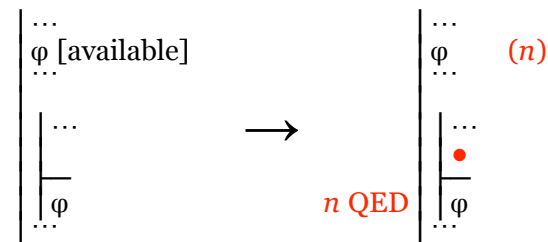
Fig. 2.2.3-3. Closing a gap by locating its goal among its resources.
