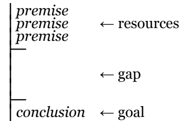
Fig. 2.2.2-1. The initial state of a derivation.
