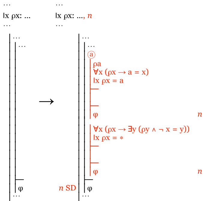
Fig. 8.6.2-1. Developing a derivation at stage n by securing a definite description; the independent term a is new to the derivation.
