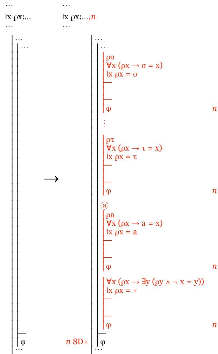
Fig. 8.6.3-1. Developing a derivation at stage n by securing a definite description; the independent term a is new to the derivation and the terms \sigma, \dots, \tau include at least one from each current alias set for the gap.
