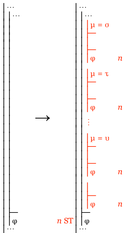
Fig. 7.8.1-2. Developing a derivation at stage n by securing a compound term \mu ; the terms \sigma, \tau, \dots, u include at least one from each current alias set for the gap.
