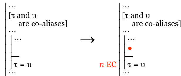
Fig. 6.3.3-1. Closing a gap whose goal is an equation between terms that are co-aliases with respect to the available resources.
