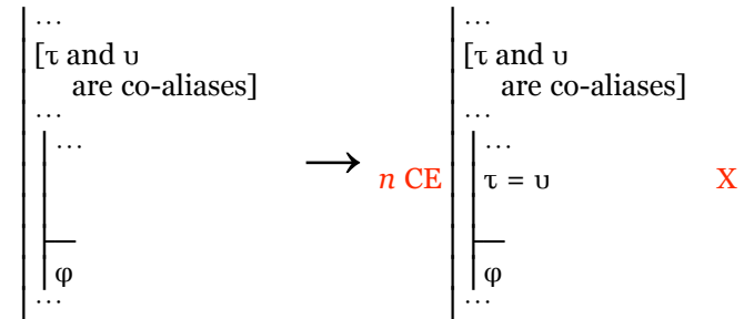
Fig. 6.3.3-5. At stage n , adding an equation between terms that are co-aliases with respect to the available resources.
