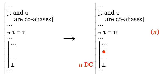
Fig. 6.3.3-2. Closing a gap of a reductio argument one of whose resources negates an equation between terms that are co-aliases with respect to the available resources.
