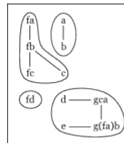
Fig. 6.3.2-4. Linked terms grouped in alias sets.
