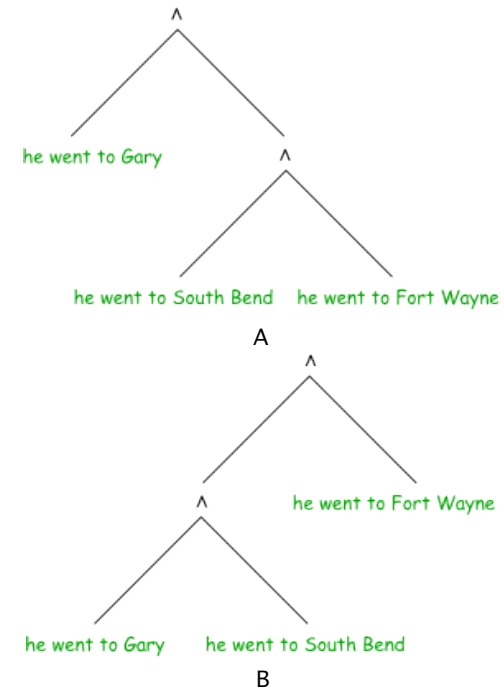
Fig. 2.1.5-1. Two analyses of a serial conjunction.
