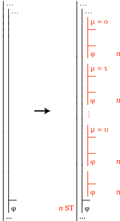
Fig. 7.8.1-2. Developing a derivation at stage n by securing a compound term \mu ; the terms \sigma , \tau , ..., \upsilon include at least one from each current alias set for the gap.
