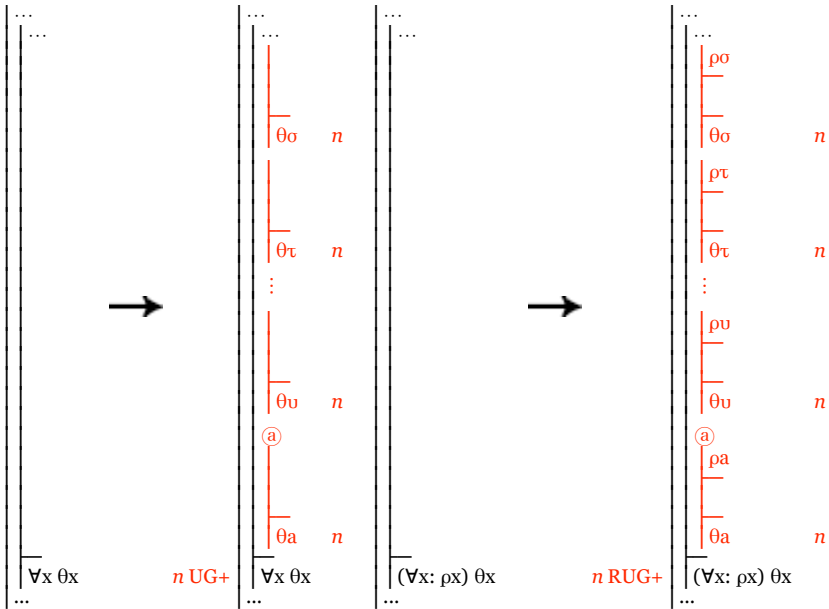
Fig. 7.8.1-1. Developing a derivation at stage n by planning for an unrestricted or restricted universal; the parameter a is new to the derivation and the terms \sigma, \tau, \dots, u include at least one from each current alias set for the gap.
